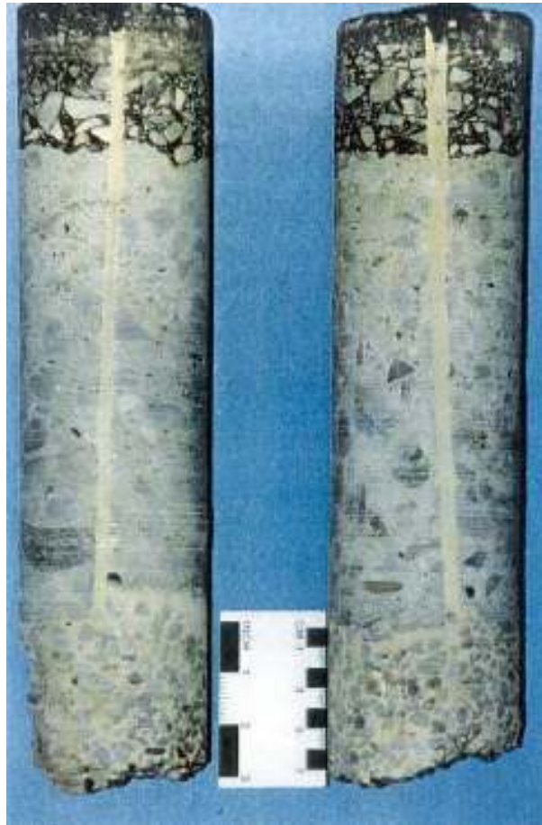
Figure 12 – View of satellite cores taken one month after installation
