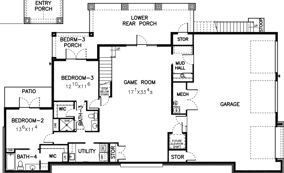
LOWER LEVEL FLOOR PLAN 1467 SQ.FT.
