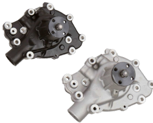
Standard rotation early water pump. 5-7/16" hub height, 5/8" shaft, 1-3/4" inlet. High flow. Available in cast or black.
