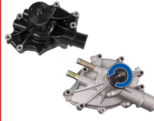
Reverse rotation 5.0L water pump ('79-93). 5-7/8" hub height, 5/8" shaft, 1-3/4" inlet. High flow. Available in cast or black.
