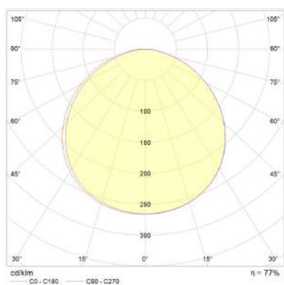
Polar curve
