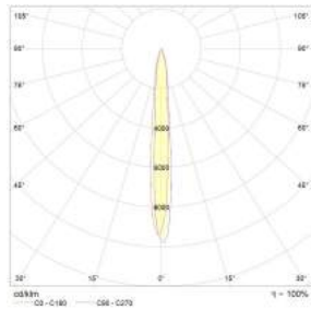
Polar Curve
