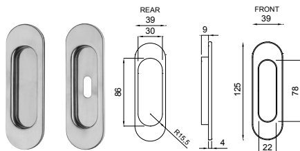
2197 placchetta incasso coprivate sliding door handle concealed fixing
