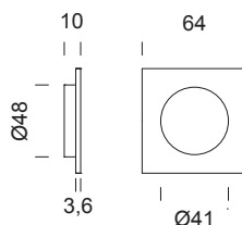
SD222 set maniglie incasso con frontale sliding door handle set with flush pull hole
