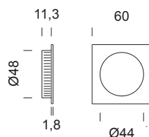
SD521 set maniglie incasso con frontale sliding door handle set with flush pull hole
