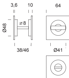
SD224 set maniglie incasso con nottolino q.8 mm. con frontale sliding door handle set with turn and release 8 mm square spindle and flush pull hole
