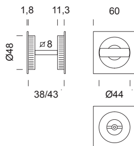
SD523M set maniglie incasso con nottolino q. 8 mm con frontale sliding door handle set with turn and release 8 mm square spindle and flush pull hole
