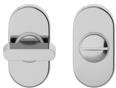
S RDN34+A set nottolino Short su rosetta stretta Short turn & release set on narrow rose 31x62mm
