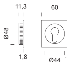
SD522Y set maniglie incasso foro yale con frontale sliding door handle set yale hole with flush pull hole
