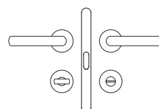
sistema Vertical con nottolino Vertical system with turn & release
