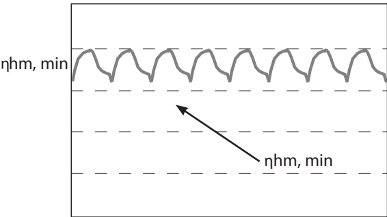
Torque at 350 bar and 2 rpm of a bent axis motor
