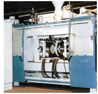
Ceramic press
